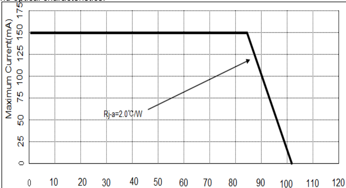
Maximum Forward Current vs. Ambient Temperature for LC25-030W-W
