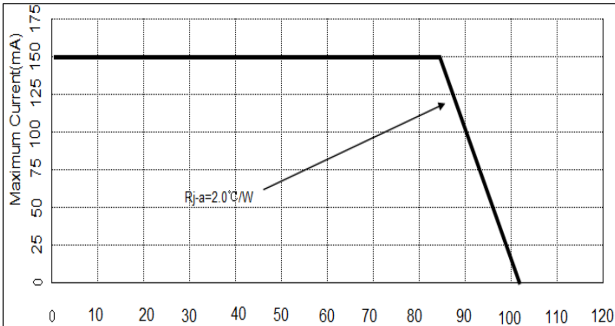
Maximum Forward Current vs. Ambient Temperature for LC35-050W-W
